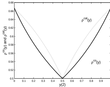
Fig. 2. \rho^{\text{cal}}(y) (dotted line) and \rho^{\text{co}}(y) (thick line) for the game of Example 2
