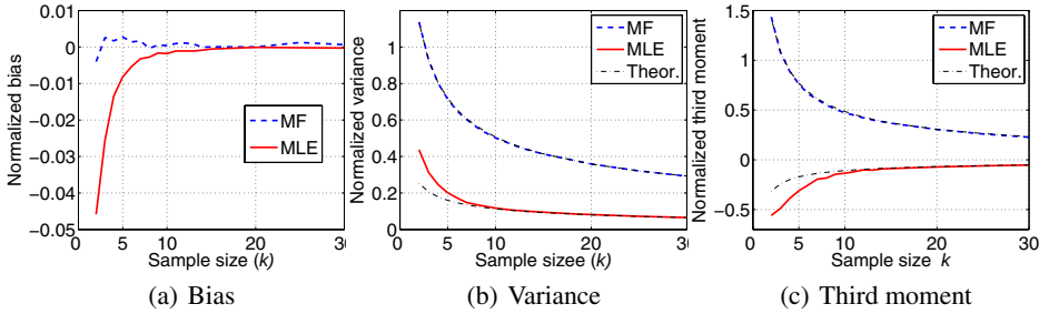
Fig. 3. Estimations of the dot products between two vectors “THIS” and “HAVE.” (a): \frac{\text{bias}}{a} , (b): \frac{\sqrt{\text{Var}(\hat{a})}}{a} , (c): \frac{3\mathbb{E}(\hat{a}-a)^3}{a} . This experiment verifies that (A): Marginal information can improve the estimations considerably. (B): As soon as k > 8 , \hat{a}_{MLE} is essentially unbiased and the asymptotic variance and third moment match simulations remarkably well. (C): The margin-free estimator ( \hat{a}_{MF} ) is unbiased and the theoretical moments are indistinguishable from simulations.
