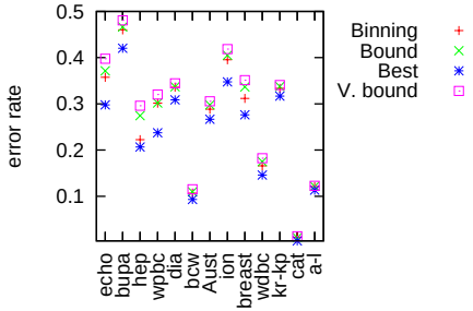
Fig. 1. In the table above we give the number of rounds, the number of experts, and the number of mistakes of the best expert. The datasets are ordered above by byte size. In the graph on the lower left we show how the performance of Binning compares to the upper Bound on Binning performance, the Best single expert, and the bound on Vovk’s algorithm. The right graph shows how the performance of Binning compares to Binomial Weighting (BW) (2 entries missing), Weighted Majority (WM), and Vovk’s algorithm.
