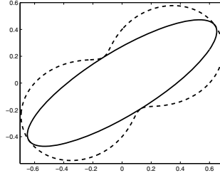
Fig. 1. An ellipse \mathcal{C} in \mathbb{R}^2 : The eigenvectors are the directions of the axes and the eigenvalues their lengths from the origin. Ellipses are weighted combinations of the one-dimensional degenerate ellipses (dyads) corresponding to the axes. (For unit \mathbf{w} , the dyad \mathbf{w}\mathbf{w}^\top is a degenerate one-dimensional ellipse which is a line between -\mathbf{w} and \mathbf{w} ). The solid curve of the ellipse is a plot of direction vector \mathcal{C}\mathbf{w} and the outer dashed figure eight is direction \mathbf{w} times the variance \mathbf{w}^\top \mathcal{C}\mathbf{w} . At the eigenvectors, this variance equals the eigenvalues and the figure eight touches the ellipse.
