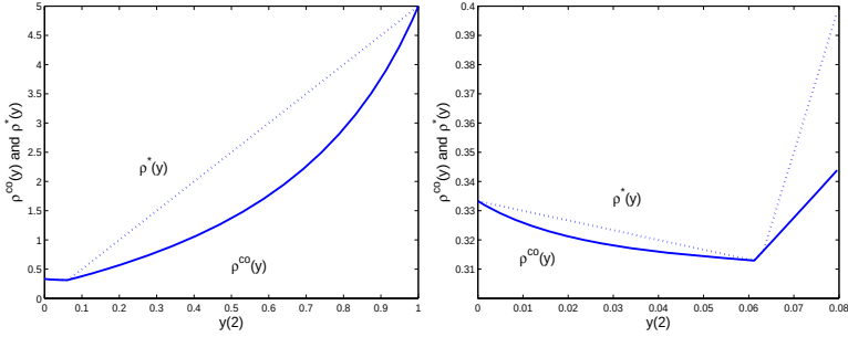
Fig. 1. \rho^*(y) (dotted) and \rho^{\text{co}}(y) (thick line) for the game of Example 1. The right figure zooms on the segment [0, 0.08] . Note that v(r, \tau) = 5/16 for that game.
